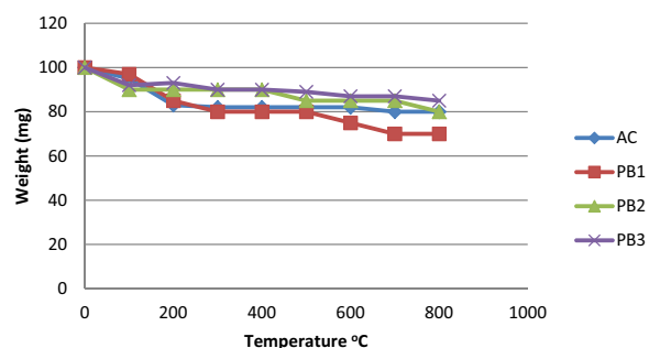
Fig. 3. Thermal stability of activated charcoal prepared via physical and chemical activation of Elaëis guineensis .
